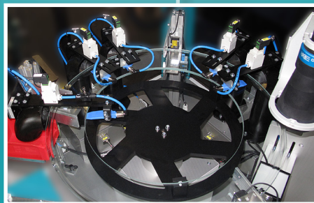
Rotary table in three different sizes
