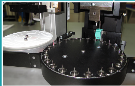
Various assembly stations integrable
